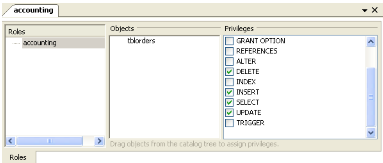
Figure 6.8. Role editor
